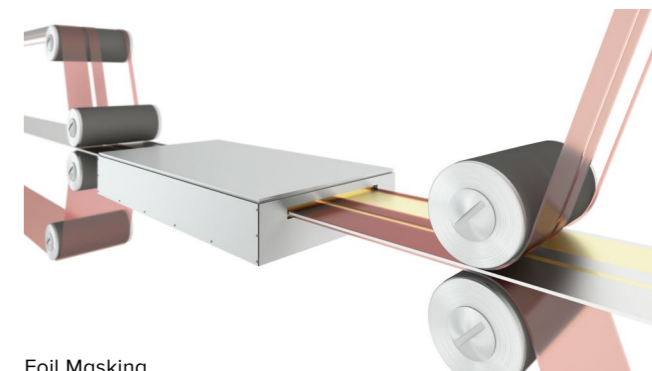
Foil Masking
