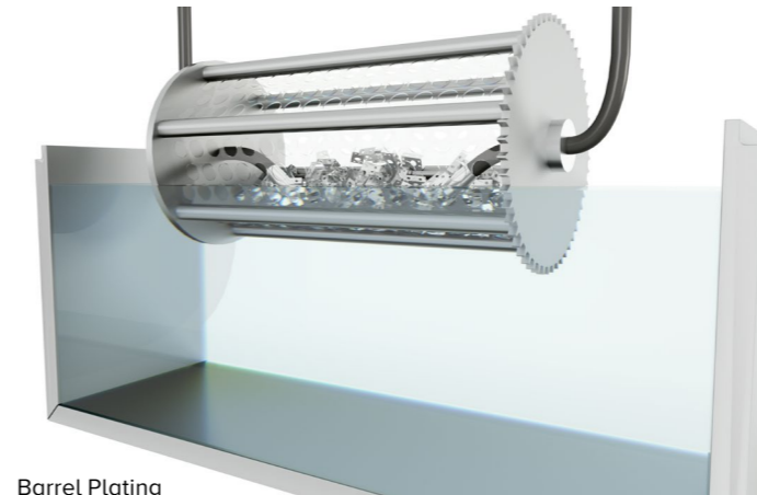
Barrel Plating
